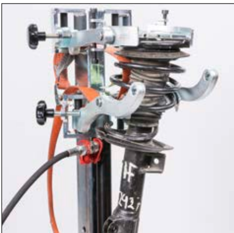
1. Change/tension springs
